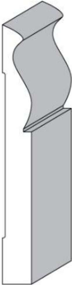
CMK 329 (5/8" x 5-1/2")
