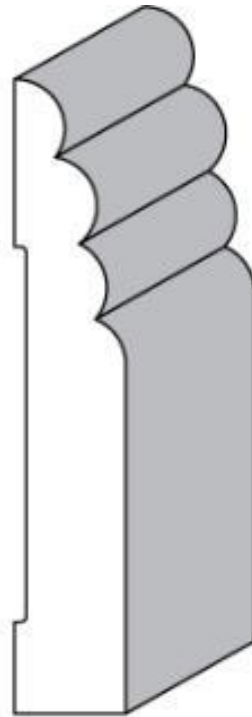
CMK 319 (11/16" x 4-1/4")
