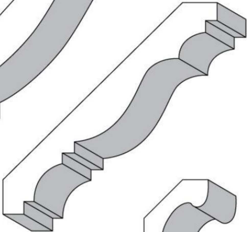
CMK 124 (7/8 " x 6-3/4")
